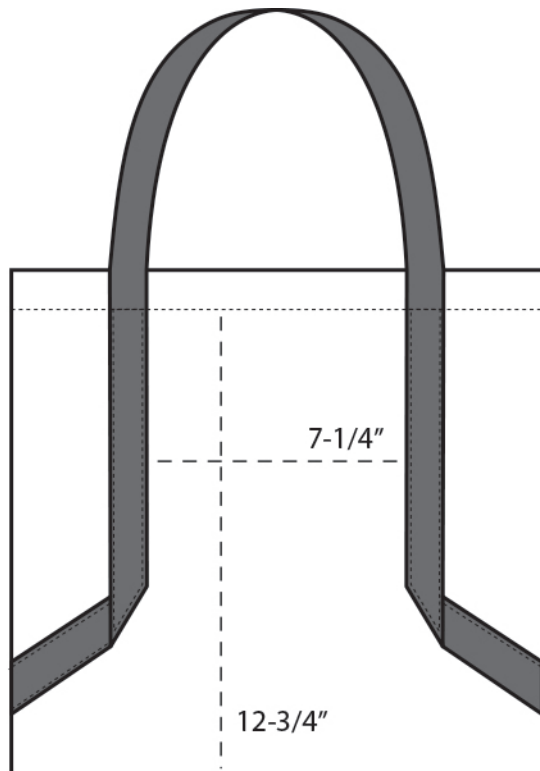
BACK VIEW
